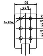
Lv bushing
